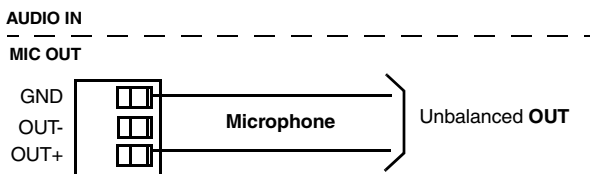
FIG. 5 Wiring the rear AUDIO IN and MIC OUT for use with Unbalanced Audio
